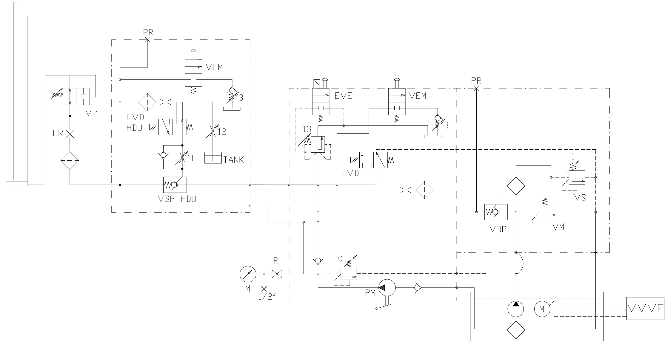
SCHEMA IDRAULICO VALVOLA HI 600+ HDU OMARLIFT - rev.01 12/04/2021 HI 600 VALVE + HDU VALVE OMARLIFT HYDRAULIC SCHEME
